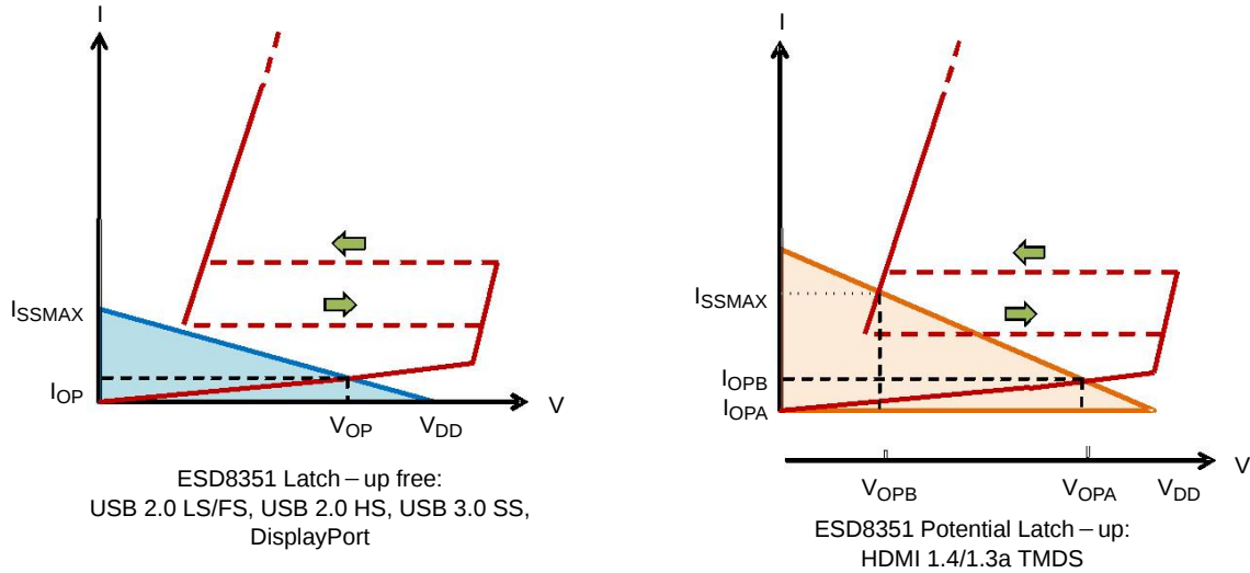
Figure 6. Example Load Lines for Latch-up Free Applications and Applications with the Potential for Latch-up
