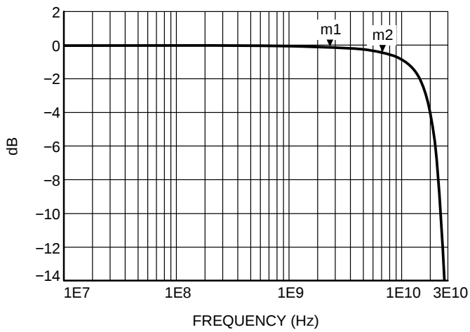
Figure 2. RF Insertion Loss
