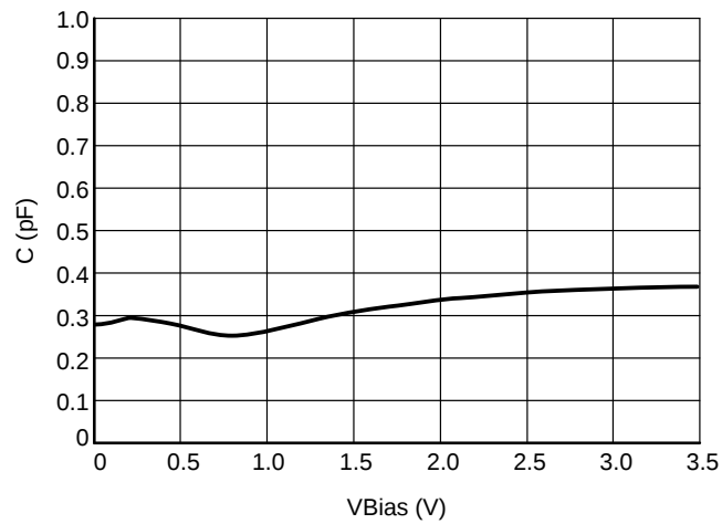
Figure 1. CV Characteristics
